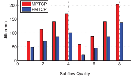
Figure 6. The average jitter of FMTCP and IETF-MPTCP. The parameters of subflow 1 remain the same (100ms delay, no packet loss). The delay and loss rate of the subflow 2 are shown in Table I.
