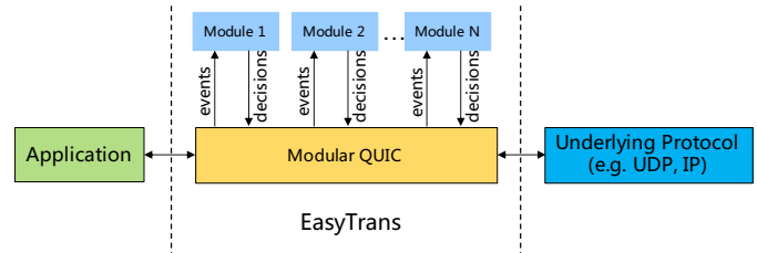
Fig. 1. EasyTrans Architecture.
